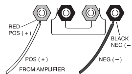
Figure 2. Series connection
