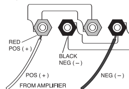
Figure 1. Parallel connection
